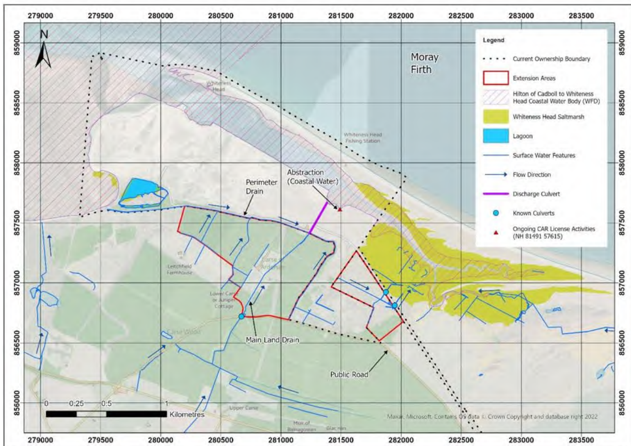
Figure 9.1: Site Layout
